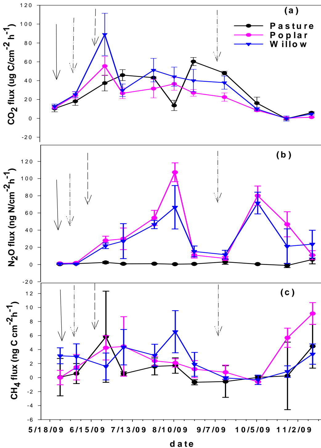
Figure 2: Fluxes of (a) CO 2 , (b) N 2 O and (c) CH 4 from the SK site for 2009. Black solid, dashed dot-dot and long dashed arrows indicate dates for herbicide application, tillage and plantation, respectively.
